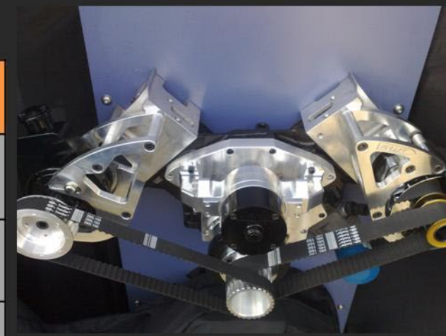
HOLDEN ALT AND POWERSTEERING BRACKETS WITH DUAL GILMER
