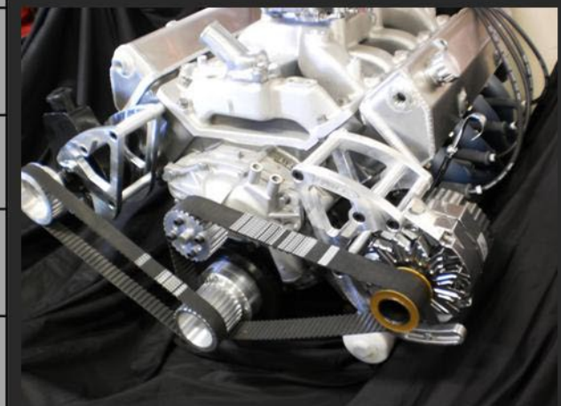
BRACKETS AND DUAL GILMER WITH MECHANICAL WATER PUMP.
